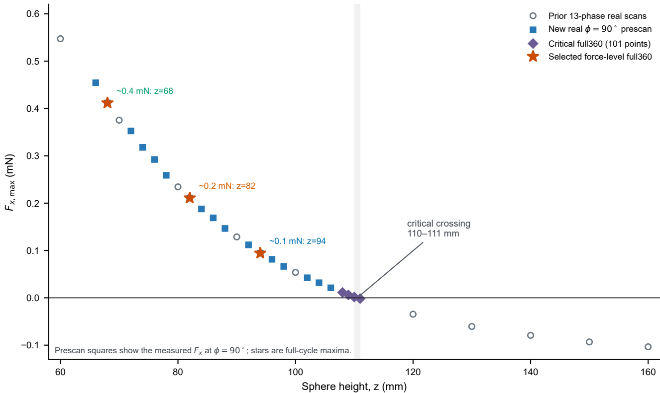
Measured force envelope versus sphere height
