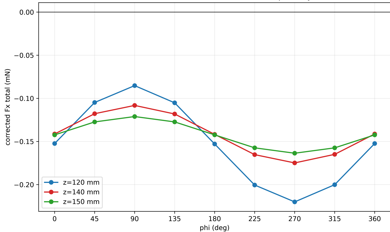
Model B: same-mesh corrected force over sparse cycle
