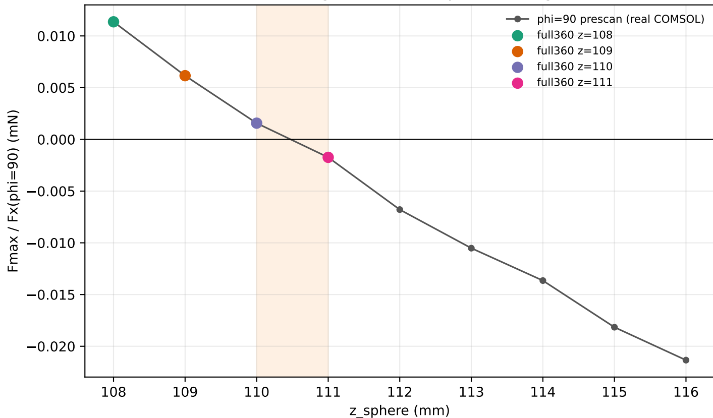
Critical sign transition, \alpha = -20^\circ
