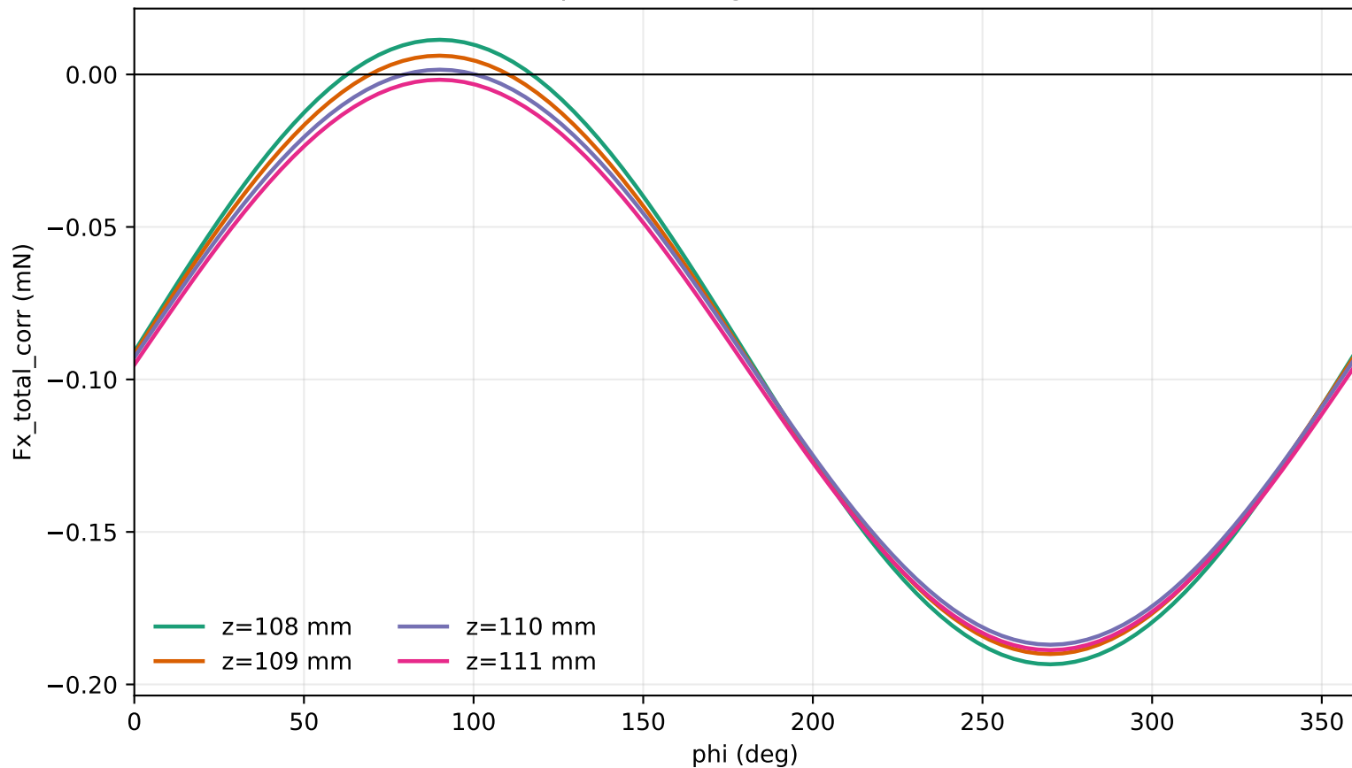
Model B alpha=-20 deg: critical full 360 curves
