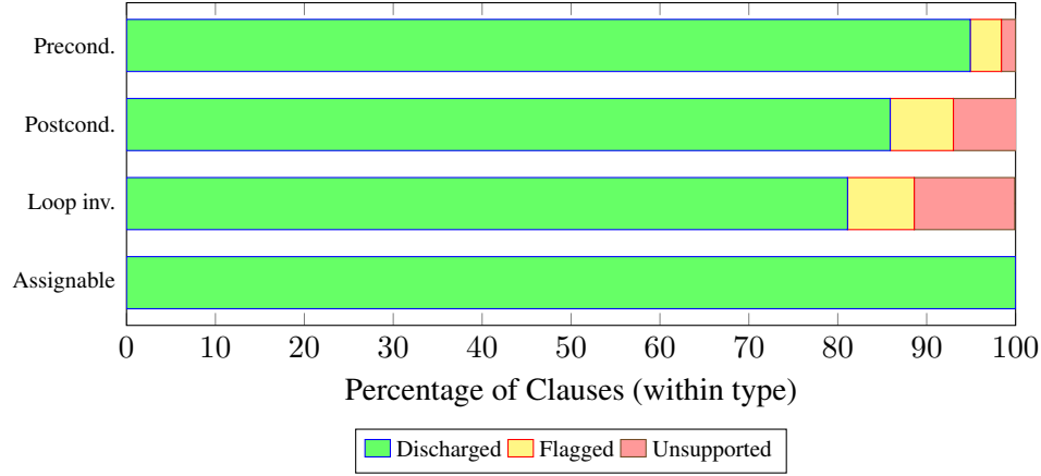
Figure 3: OpenJML discharge outcome by inferred-clause type, visualising Table 3. The 7.1% postcondition unsupported rate is concentrated in nested-quantifier \backslash_{\text{sum}} clauses; the 11.3% loop-invariant unsupported rate covers inductive accumulator forms that exceed Z3’s tractability budget (Section 6).
