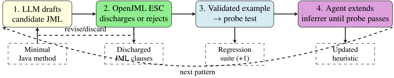
Figure 2: Probe-and-backport development loop . An LLM proposes candidate JML for a target code pattern; OpenJML’s ESC discharges or rejects each clause under the fixed strictness configuration of Section 3.2; validated examples are pinned as probe tests in the verification regression suite; an agentic coding assistant then extends the appropriate inference component until the probe passes without regressing existing probes. The verifier is the non-negotiable filter on what the LLM is allowed to teach the inferer.
