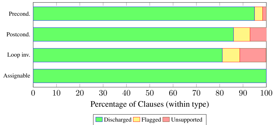
Figure 3: OpenJML discharge outcome by inferred-clause type, visualising Table 3. The 7.1% postcondition unsupported rate is concentrated in nested-quantifier \sum clauses; the 11.3% loop-invariant unsupported rate covers inductive accumulator forms that exceed Z3’s tractability budget (Section 6).
