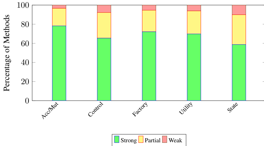
Figure 4: Distribution of specification strength by method category over the 312-method corpus. Strong specifications have non-trivial preconditions and postconditions; partial have exactly one non-trivial side; weak have neither. Bars sum to 100% within category.
