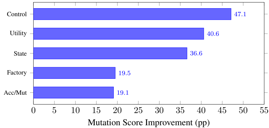
Figure 5: Improvement in mutation score (percentage points) from P1 to P3 by method category. The other category is omitted (zero methods in the corpus).
