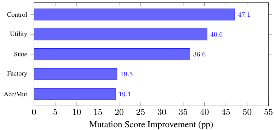
Figure 3: Improvement in mutation score (percentage points) from P1 to P3 by method category. The other category is omitted (zero methods in the corpus).
