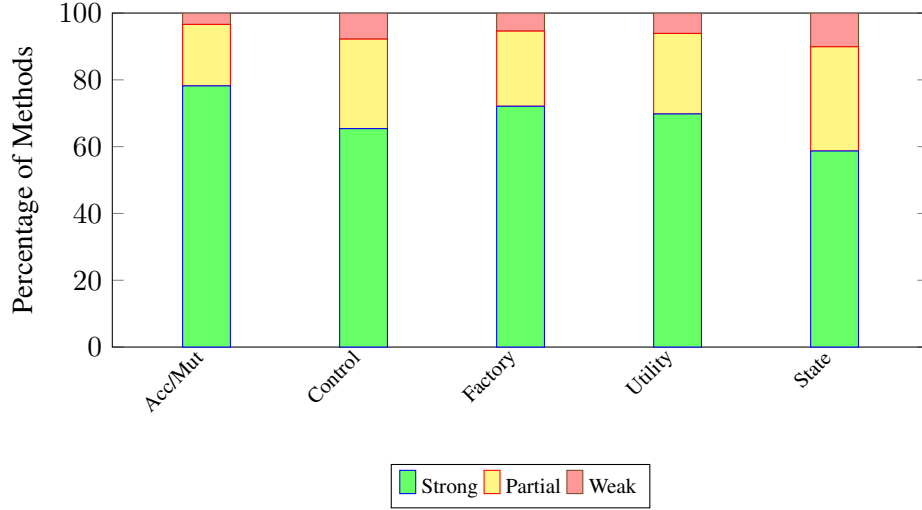
Figure 2: Distribution of specification strength by method category over the 312-method corpus. Strong specifications have non-trivial preconditions and postconditions; partial have exactly one non-trivial side; weak have neither. Bars sum to 100% within category.
