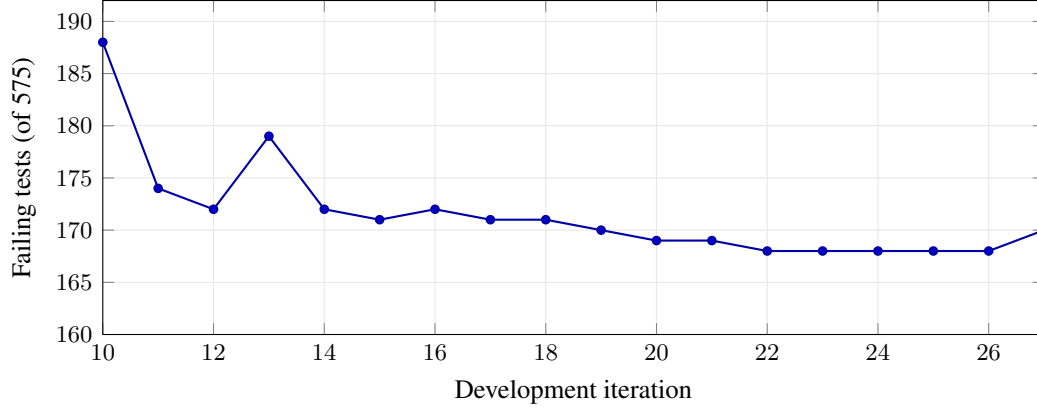
Figure 3: Effect of the probe-and-backport loop over one development window in which the end-to-end verification suite was held fixed at 575 tests. Backporting validated probes reduced failing tests from 188 at the start of the window to a plateau of 168; the upward steps (notably at iterations 13 and 27) are candidate heuristics that regressed the suite under the fixed strictness configuration and were reverted before the next iteration. Each test asserts that the inferer, given a bare method, emits a specification that OpenJML’s ESC discharges. Iterations are numbered by their position in the project’s fix sequence (fix10–fix27). Later iterations expanded the suite with further probes and are not shown, as the changing denominator makes raw failing-test counts non-comparable across the full history.
