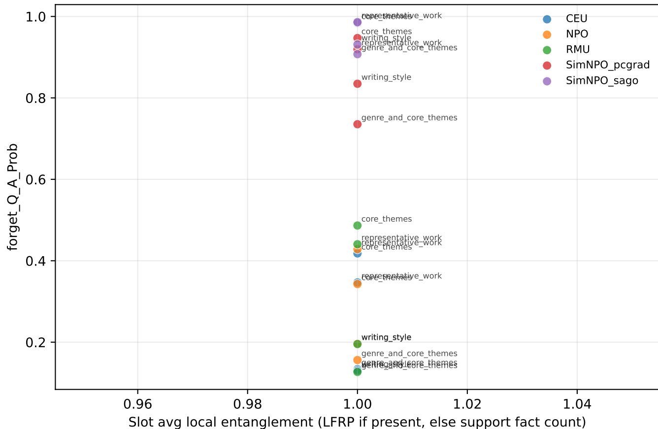
Slot Entanglement vs Forget Leakage
