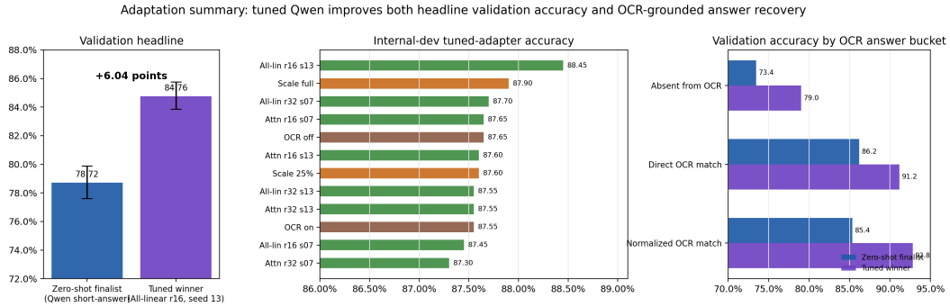
Figure 3: Adaptation summary. Left: the final tuned Qwen model improves validation accuracy by 6.04 points over the strongest zero-shot finalist. Middle: internal-dev post-train accuracy across the full 12-run LoRA study, including the core matrix and winner-conditioned follow-ups. Right: validation gains are largest for OCR-grounded answers, especially those that require normalized OCR matching.
