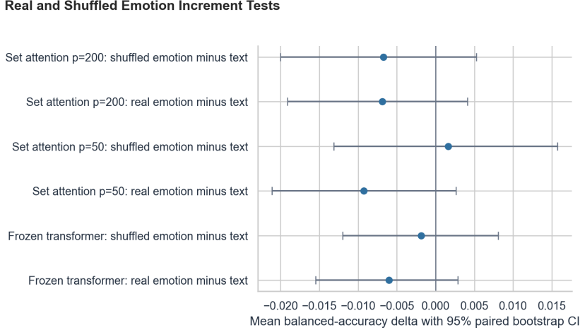
Figure 3: Real-emotion and shuffled-emotion deltas vs. text-only, with 95% paired bootstrap CIs over test authors. Across all three families (frozen MiniLM probes, set-attention P=50 , set-attention P=200 ), the real-emotion CI overlaps the shuffled-emotion CI and both straddle zero. The negative-control logic implies emotion does not add robust incremental signal beyond text.
