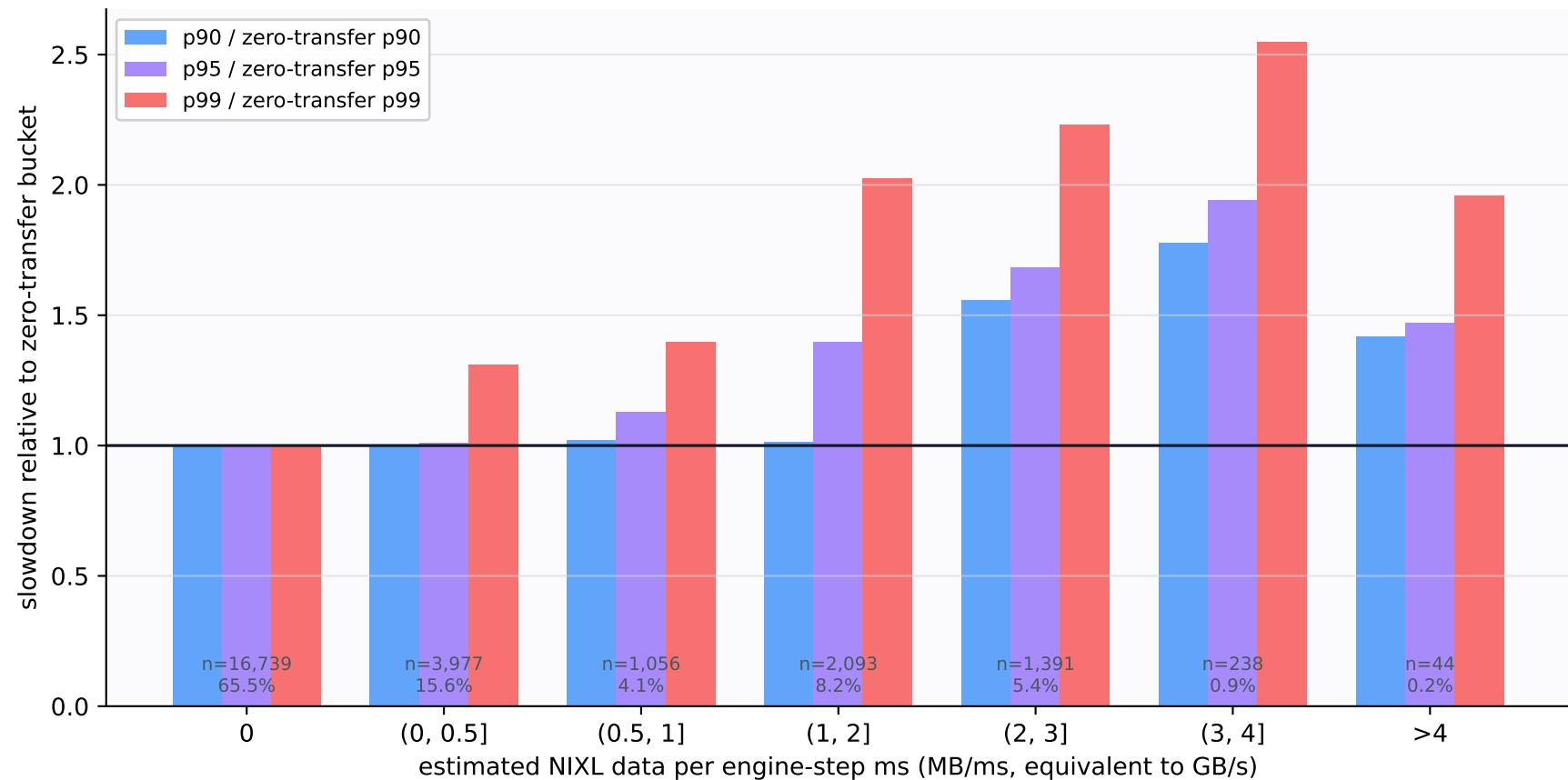
Main Run: engine-step Tail Slowdown vs Normalized In-Step Transfer Volume
