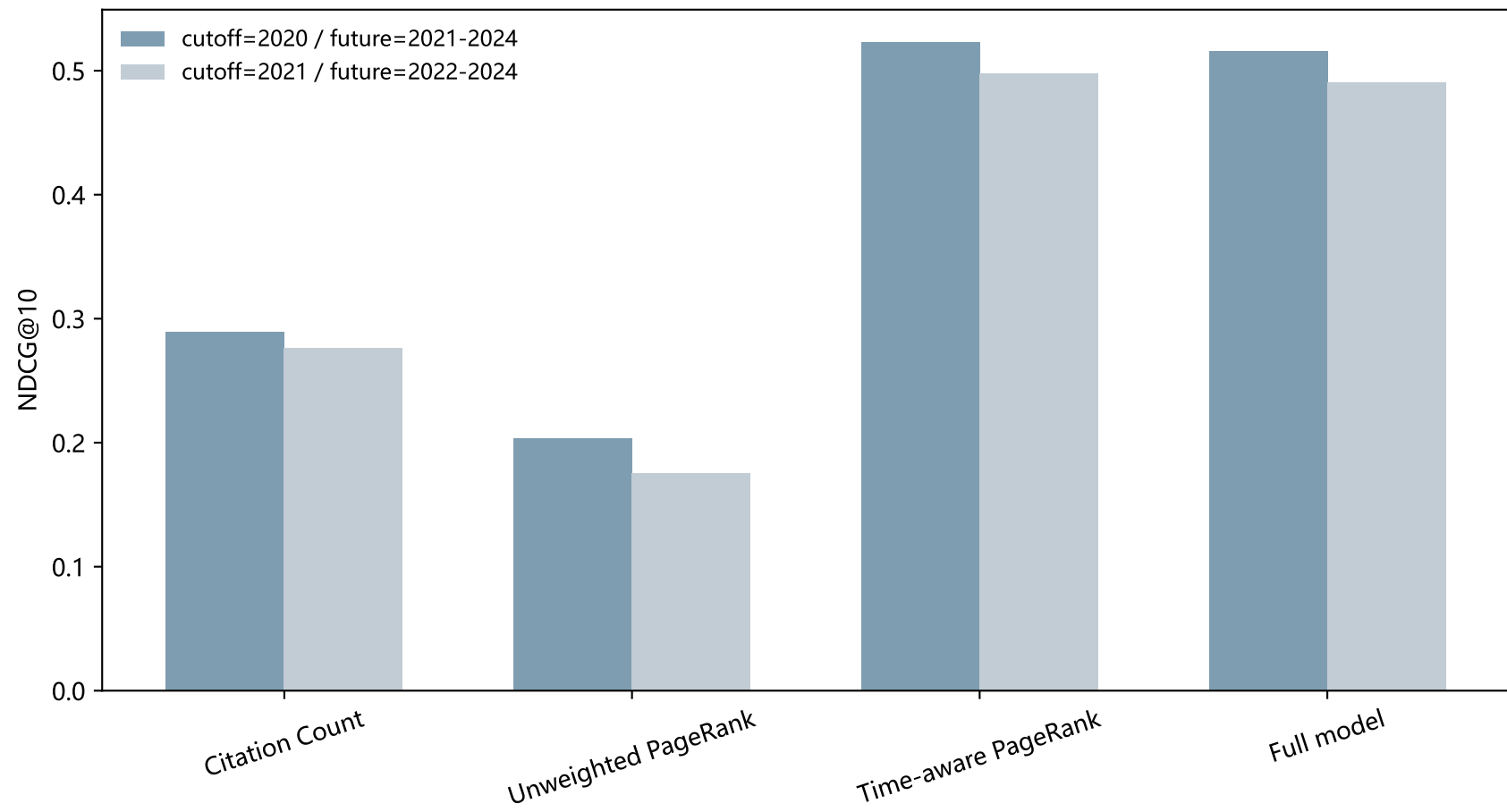
Future citation validation: NDCG@10 对比
