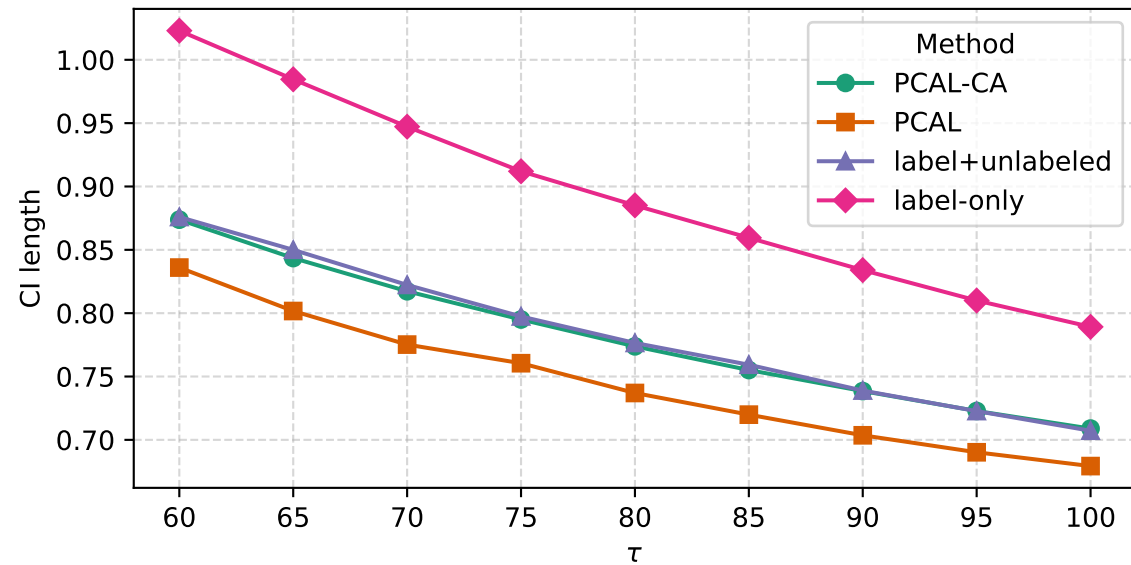
Lengths of confidence intervals with varying \tau
