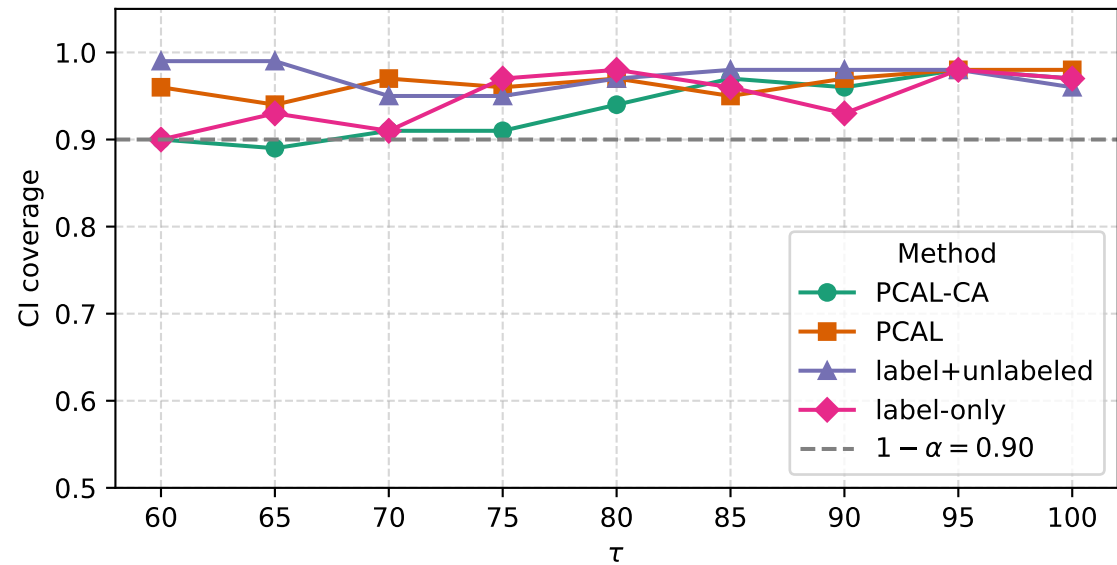
Coverage of confidence interval with varying \tau
