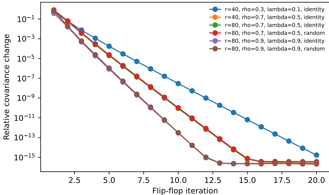
Regularized flip-flop iterations stabilize rapidly
