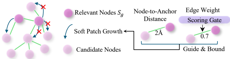
Figure. P1: Illustration of the two components in the adaptive compression analysis. (a) Smallest-cardinality budget selection by sorting node relevance scores and choosing the minimal anchor set S_g whose cumulative mass reaches the threshold \rho ; (b) soft patch growth from relevant anchors to nearby candidate nodes, guided by node-to-anchor distance and edge-based scoring.
