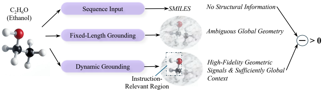
Figure. P4: Illustration of the geometry-grounding argument under three input conditions. The top branch uses sequence alone, the middle branch uses fixed-length grounding, and the bottom branch uses dynamic grounding over the instruction-relevant region, showing the different levels of structural information retained before prediction.
