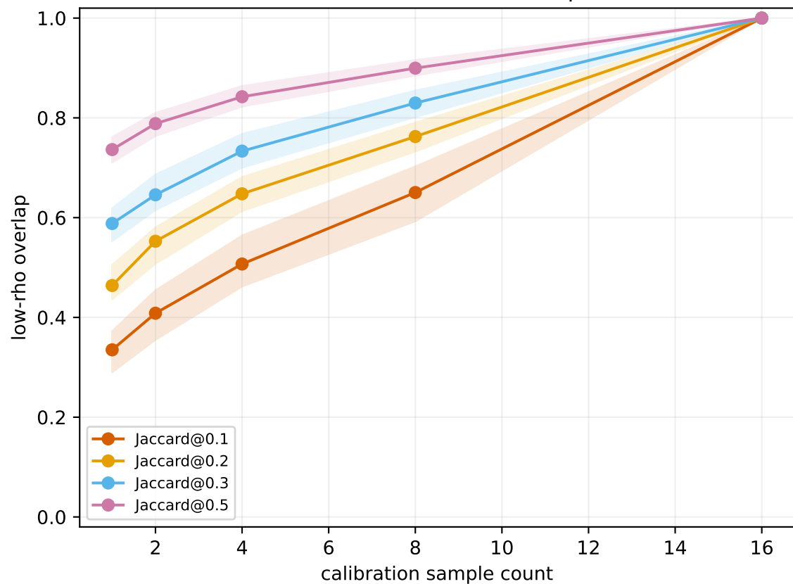
Low-rho selection overlap
