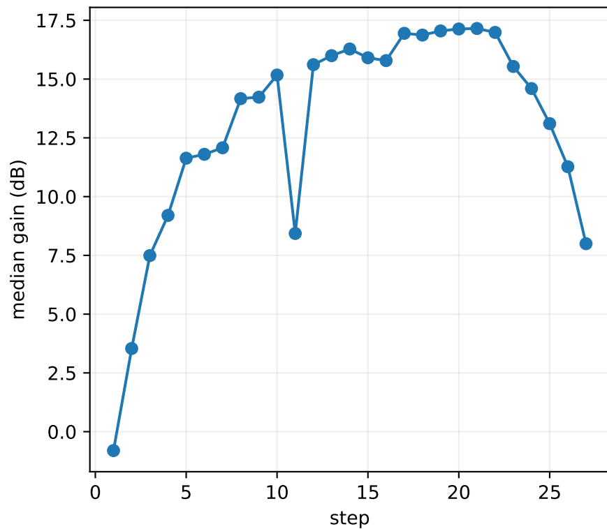
FLUX
