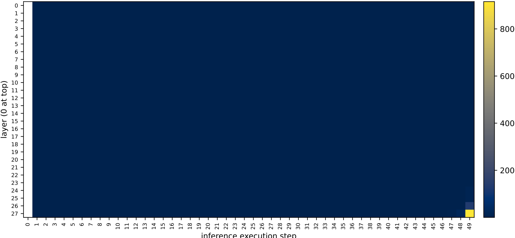
DIT \log_{10} V(\text{diff})
