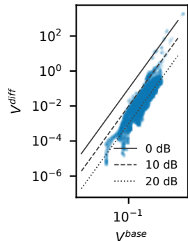
C Aligned vs. shuffled
