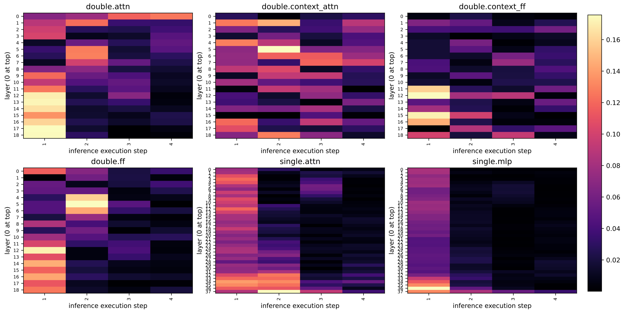
FLUX log_rho_mad by module
