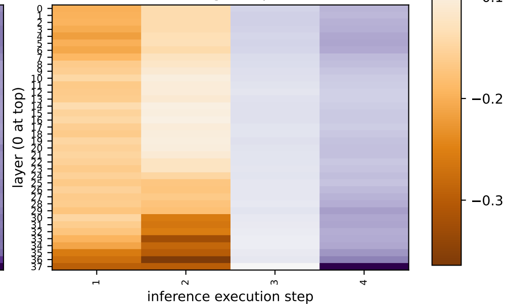
single.mlp
