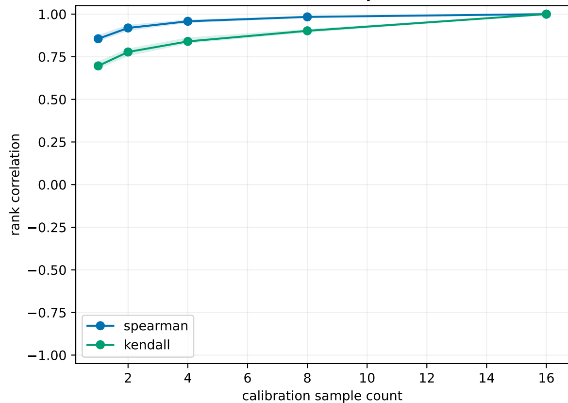
Rank stability
