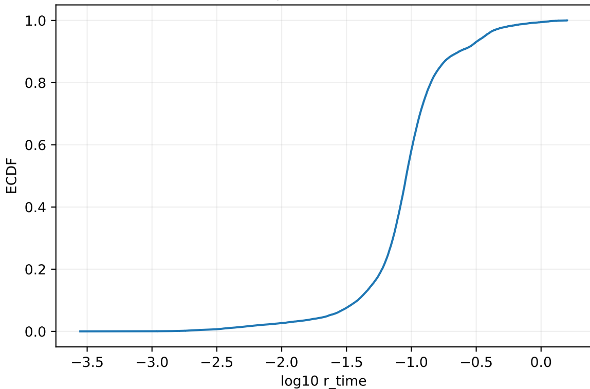
Temporal rate ECDF
