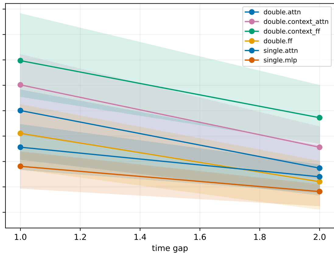
CCMR time-gap ablation by model and module
