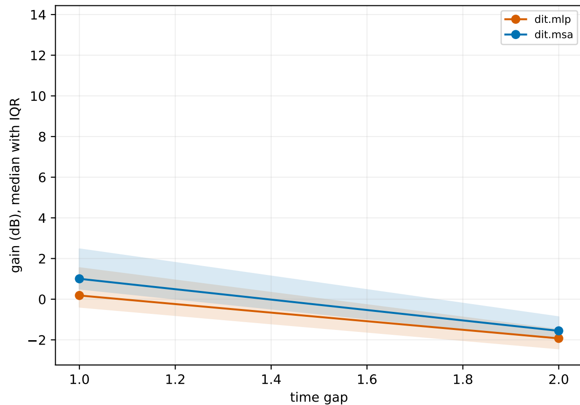
CCMR time-gap ablation by model and module
