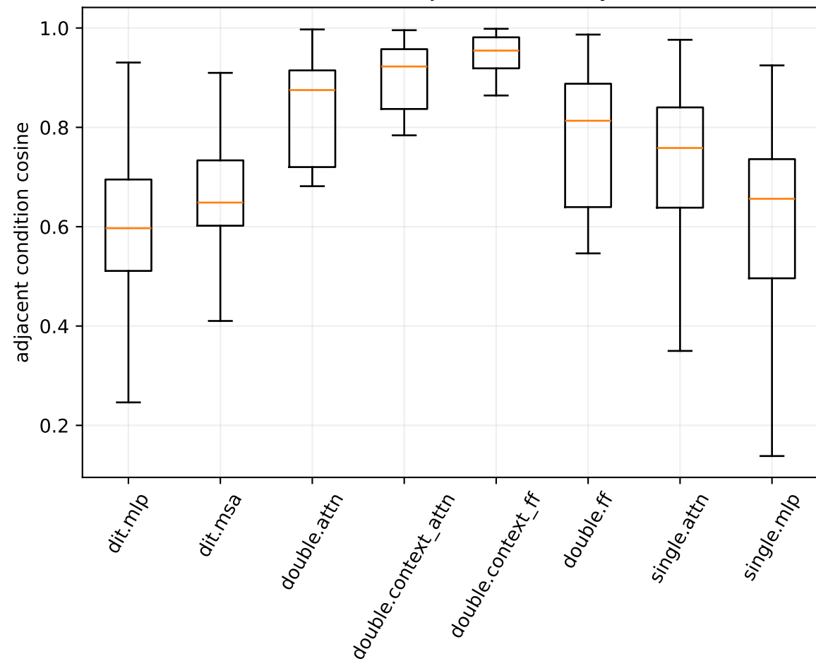
Condition adjacent similarity
