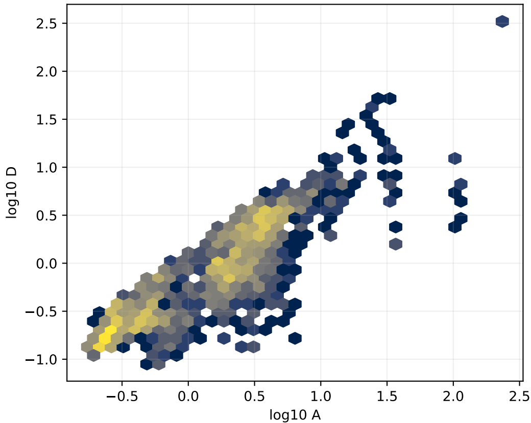
Temporal smoothness
