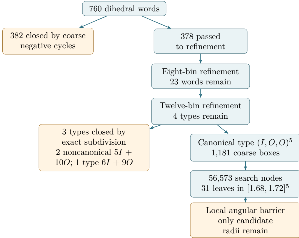
Figure 5: The replayed reduction path. Unlike an earlier exploratory gap-capacity filter, the certified path tests all 760 dihedral classes directly; the counts here match the included verifier reports.
