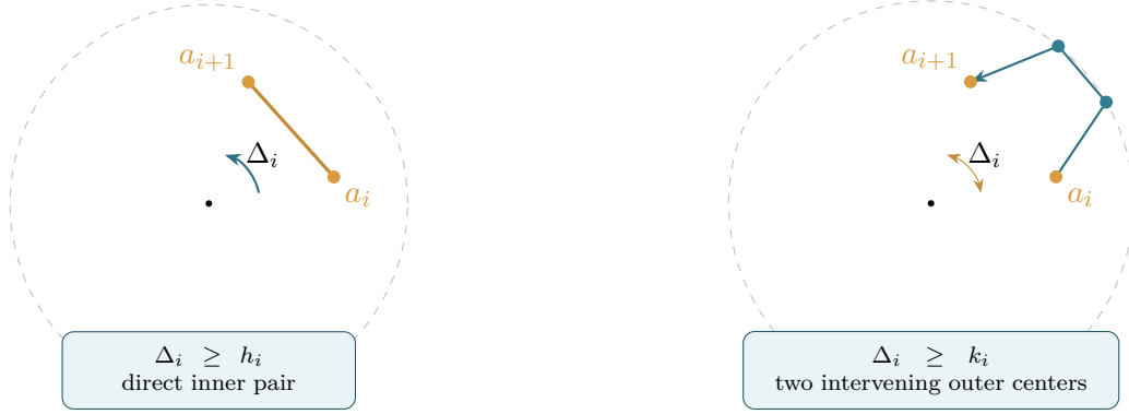
Figure 6: Each inner-to-inner sector has two independent lower bounds. Combining them gives \Delta_i \geq \max\{h_i, k_i\} , which leads to the total angular budget in equation (6) . The radii and angles are schematic.
