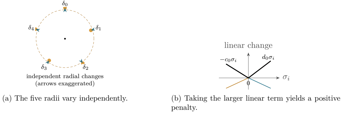
Figure 7: The local barrier has no hidden symmetry constraint: radial deviations are independent, while the maximum of the oppositely sloped first-order terms grows away from \sigma_i = 0 . Quadratic errors are controlled by the exact interval bounds.
