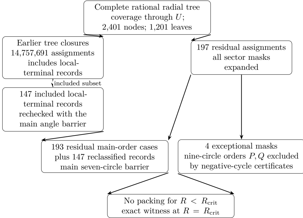
Figure 3: The finite lower-bound proof. The dashed arrow marks the 147 local-terminal records as a subset of the earlier closure count; they are rechecked through the main angle barrier and are not extra sector assignments. The case rules exclude hypothetical packings below R_{\text{crit}} , while the exact witness attains the boundary value.
