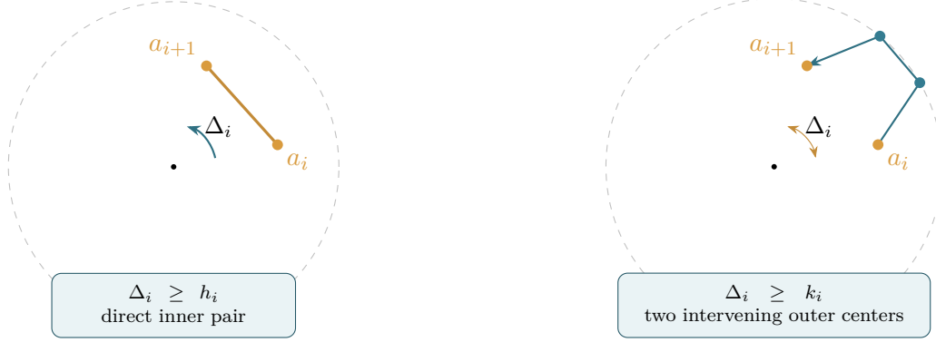
Figure 9: Each inner-to-inner sector has two independent lower bounds. Combining them gives \Delta_i \geq \max\{h_i, k_i\} , which leads to the total angular budget in equation (6) . The radii and angles are schematic.
