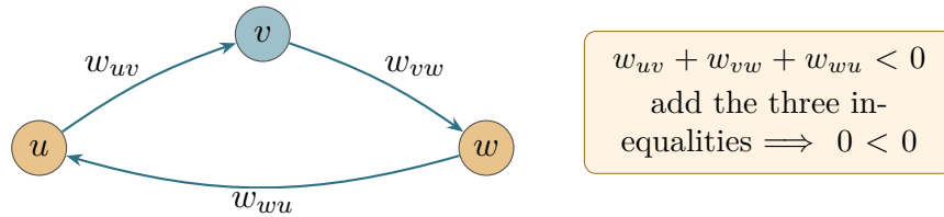
Figure 5: A negative directed cycle is a compact contradiction: summing its difference inequalities cancels all angle variables. The actual verifier uses exact integer edge weights for each radial box.
