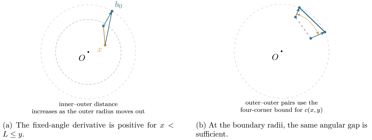
Figure 2: Schematic of the wall-pushing argument. The left panel is monotonicity of squared distance; the right panel summarizes lemma 3.1 . The dashed pair is illustrative, not a pointwise distance comparison throughout simultaneous motion.
