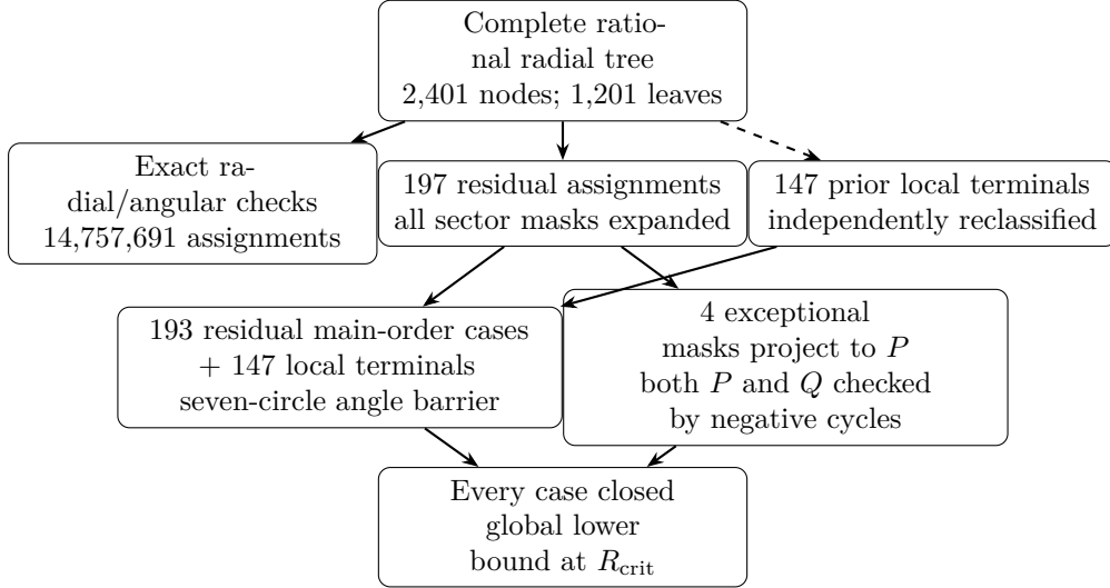
Figure 1: Structure of the finite lower-bound proof. The 147 local terminals are a separate set of tree conclusions, rechecked through the main angle barrier; they are not additional sector assignments.
