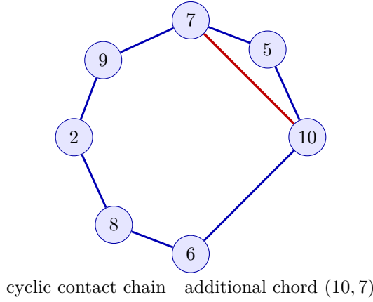
Figure 2: Contact graph of the seven-circle core. The blue cycle contributes seven tangencies; the red chord is the eighth core tangency.
