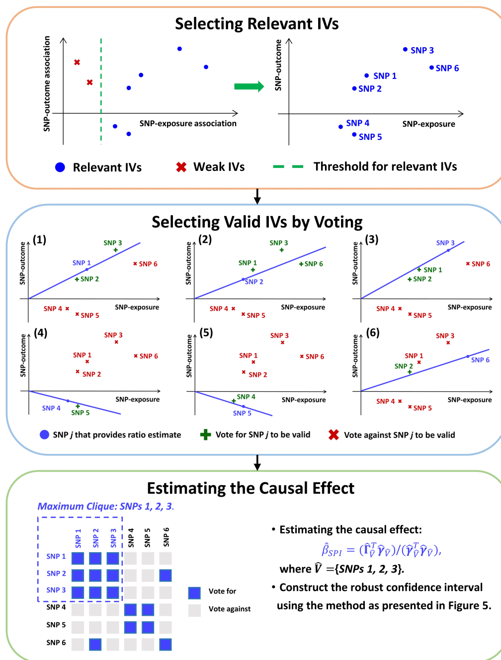
Figure 1: The MR-SPI framework. First, MR-SPI selects relevant IVs with strong SNP-exposure associations. Second, each relevant IV provides a ratio estimate of the causal effect and then receives votes on itself to be valid from the other relevant IVs whose degrees of violation of (A2) and (A3) are small under this ratio estimate of causal effect. For example, by assuming SNP 1 is valid, the slope of the line connecting SNP 1 and the origin represents the ratio estimate of SNP 1, and SNPs 2 and 3 vote for SNP 1 to be valid because they are close to that line, while SNPs 4, 5 and 6 vote against it since they are far away from that line. Third, MR-SPI estimates the causal effect by fitting a zero-intercept OLS regression of SNP-outcome associations on SNP-exposure associations and construct the robust confidence interval using selected valid SNP IVs in the maximum clique of the voting matrix, which encodes whether two SNPs mutually vote for each other to be valid IVs.
