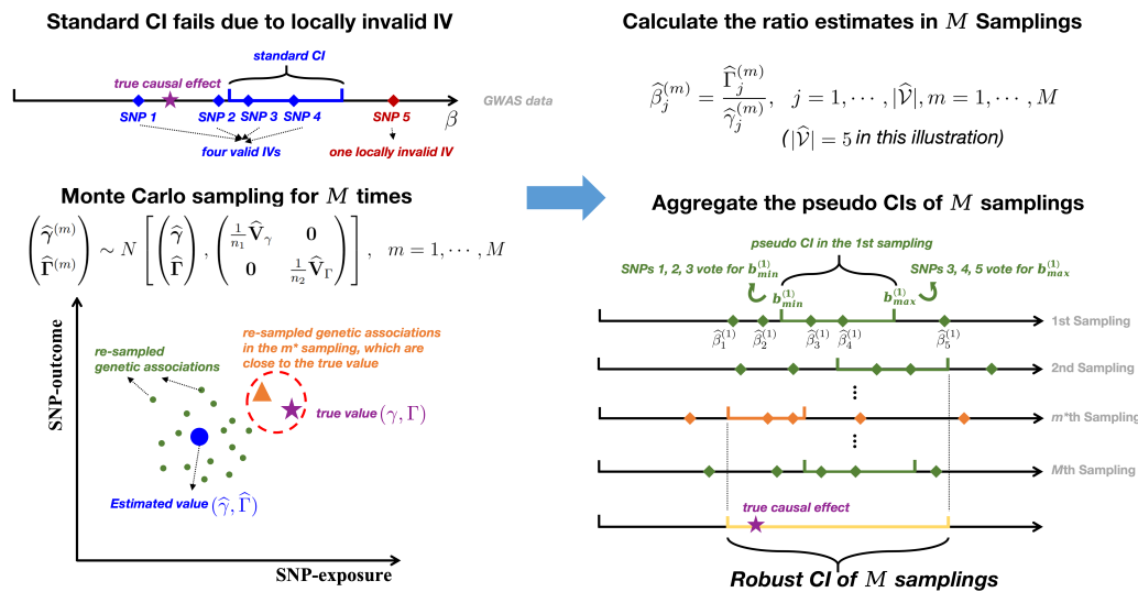
Figure 5: The proposed procedure for constructing the robust confidence interval by MR-SPI that allows for finite-sample IV selection error. When Locally invalid IVs may be exist in finite samples, MR-SPI might incorrectly selected invalid IVs as valid ones (marked by the red cross) in finite-sample settings, and thus the standard CI might fail to cover the true causal effect. First, we construct an initial interval using SNPs in and discretize it to a grid set. Second To deal with this issue, we repeatedly sample the estimators of \gamma and \Gamma for M times (by default, we set M = 1,000 ) from the sampling distribution. When M is sufficiently large, there exists m^* th sampling such that the re-sampled genetic associations (marked by orange triangle) are close enough to the true values \gamma and \Gamma . In each sampling, we calculate the ratio estimates using the re-sampled genetic associations, and then construct a pseudo CI for the causal effect by line searching. Specifically, for any value b in the pseudo CI, more than half of the IVs selected by MR-SPI (in this illustration, at least three IVs) should vote for b to be the true causal effect. We then aggregate all the pseudo CIs of M samplings by taking the minimum of the lower bounds and the maximum of the upper bounds to construct the robust CI (marked by yellow segment).
