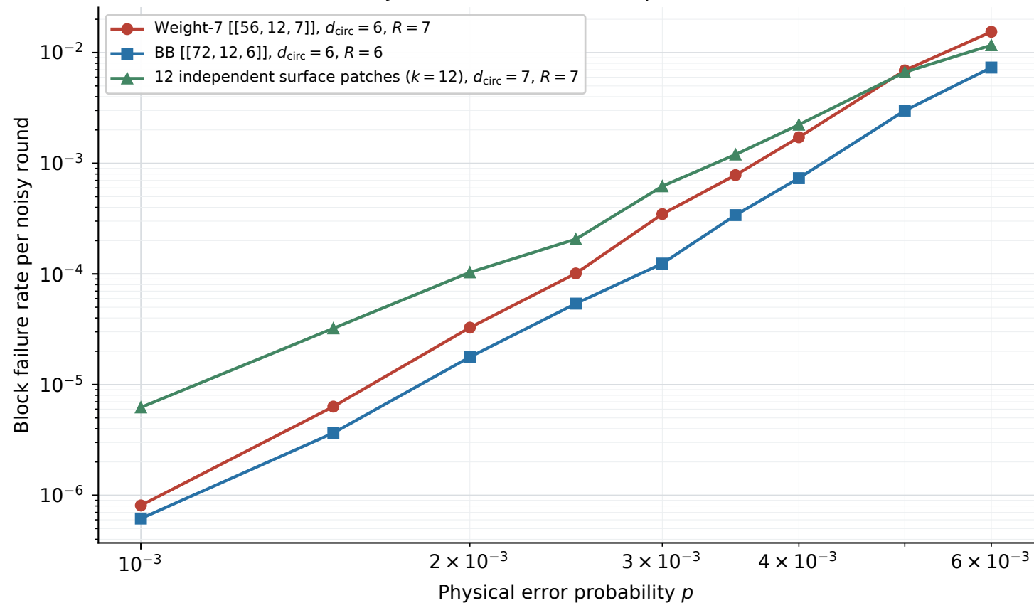
Joint X/Z block failure: equal k=12
