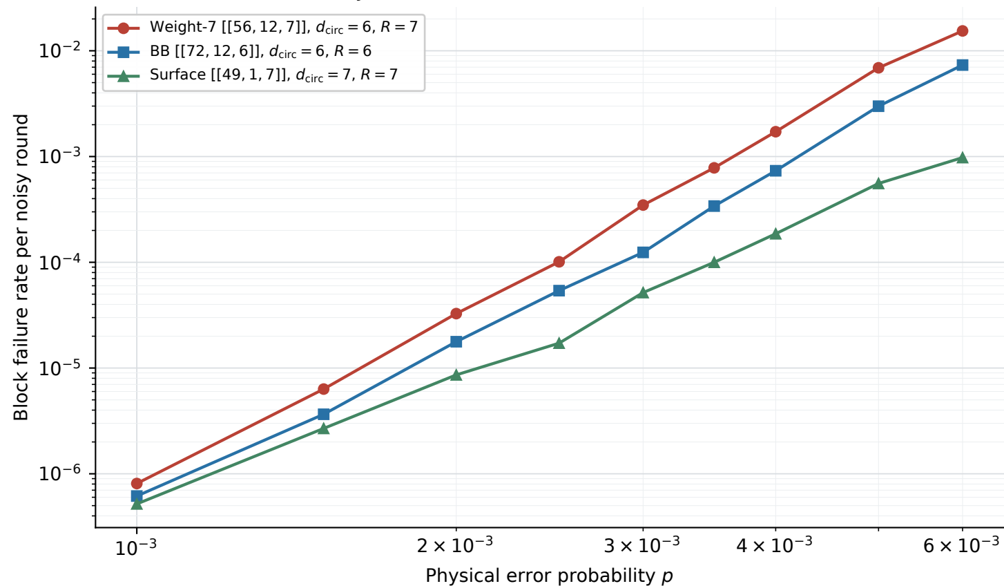
Joint X/Z block failure: one code block
