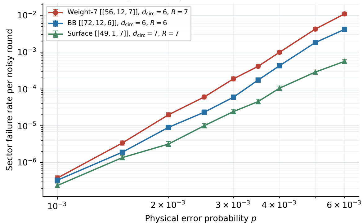
Logical Z component: one code block
