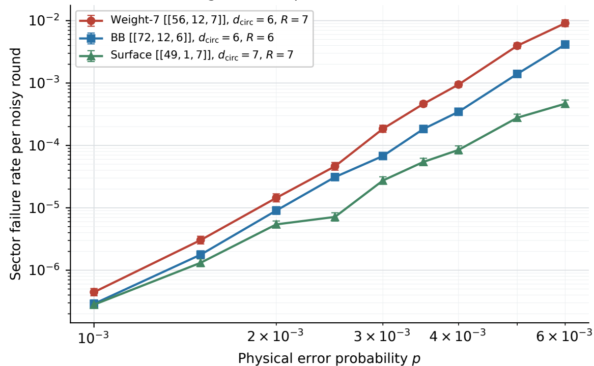
Logical X component: one code block
