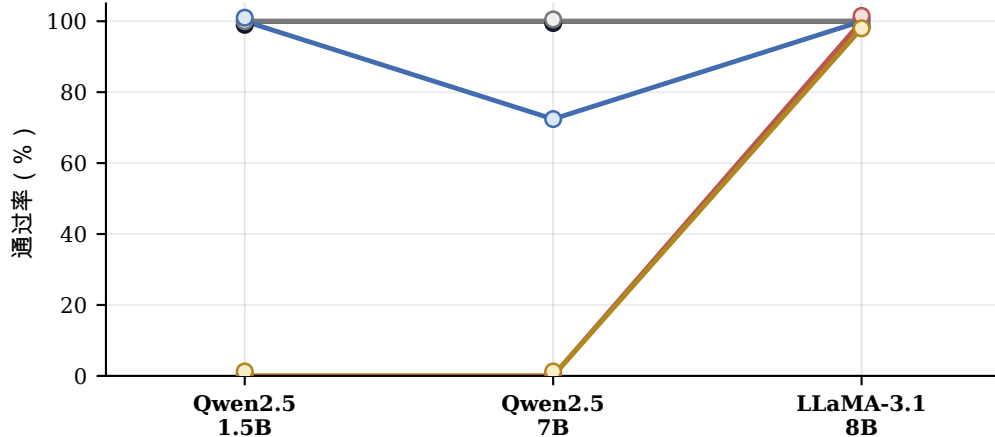
(a) Needle
