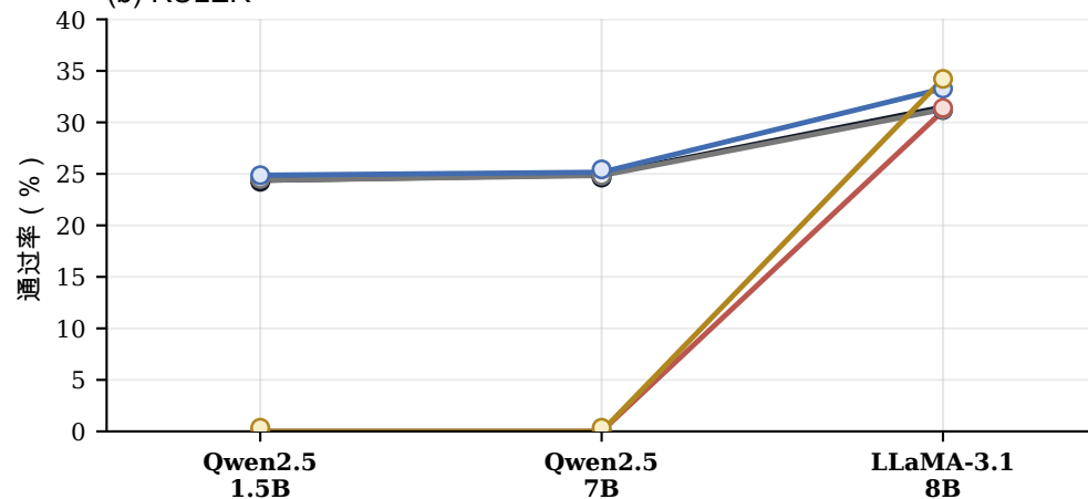
(b) RULER
