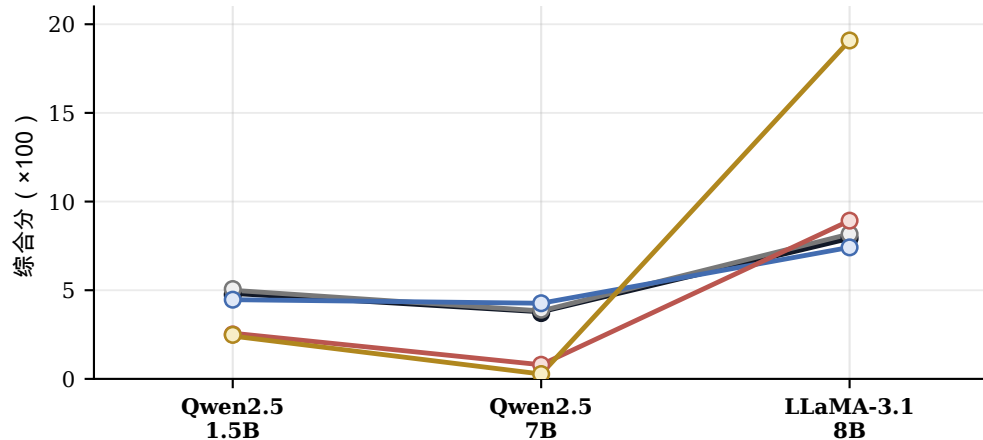
(c) LongBench
