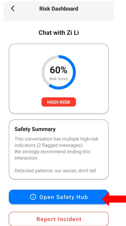
Figure 17 Risk Dashboard
