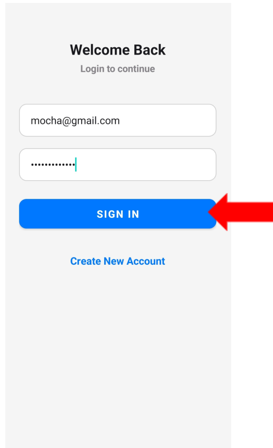
Figure 12 Login Screen
