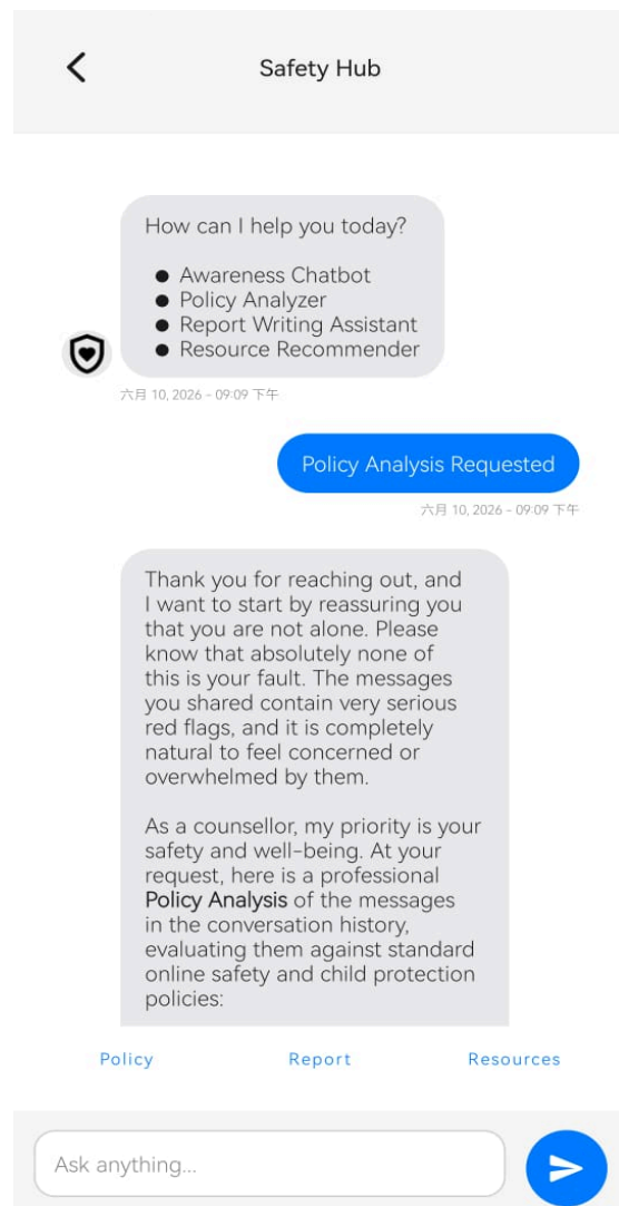
Figure 19 Policy
