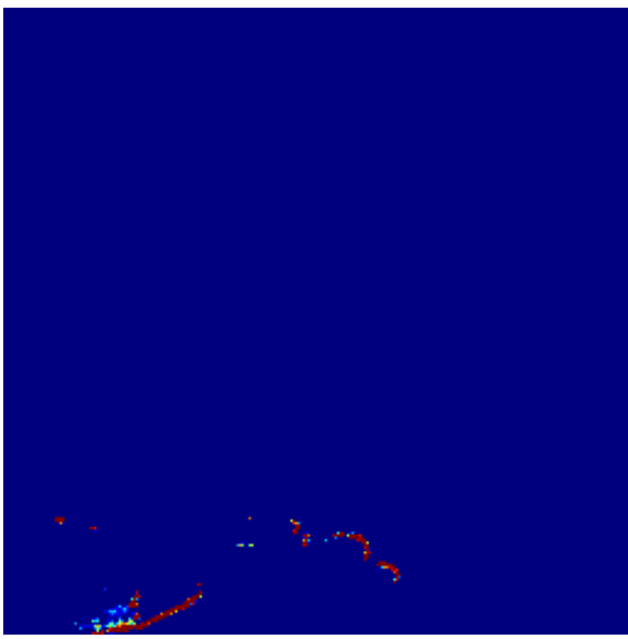
Baseline+BCE
