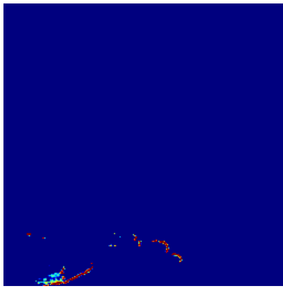
Baseline+SFL
