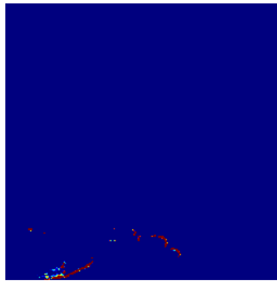
DualSight-Fire+BCE
