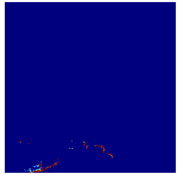
DualSight-Fire+SFL
