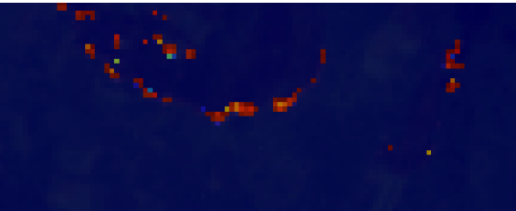
DualSight-Fire+BCE
