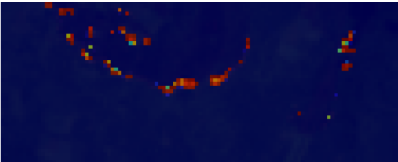
Baseline+BCE
