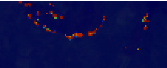
Baseline+SFL
