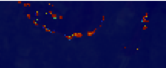
DualSight-Fire+SFL
