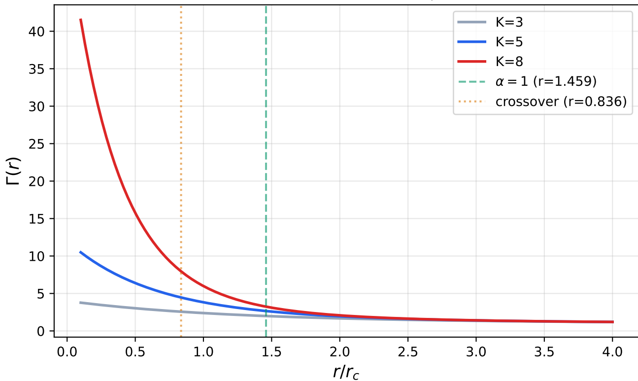
FibonacciVortex circulation profile
