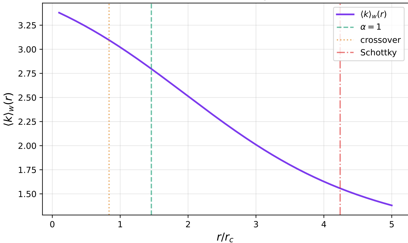
Effective mode index (Burgers strain)
