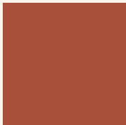
four equal sides
