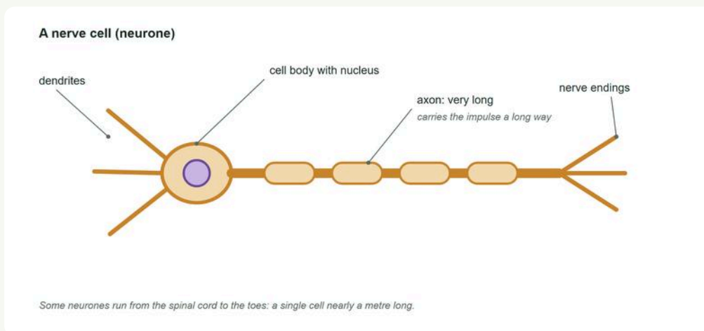
Figure 1.8 A nerve cell. The axon may be very long indeed.
