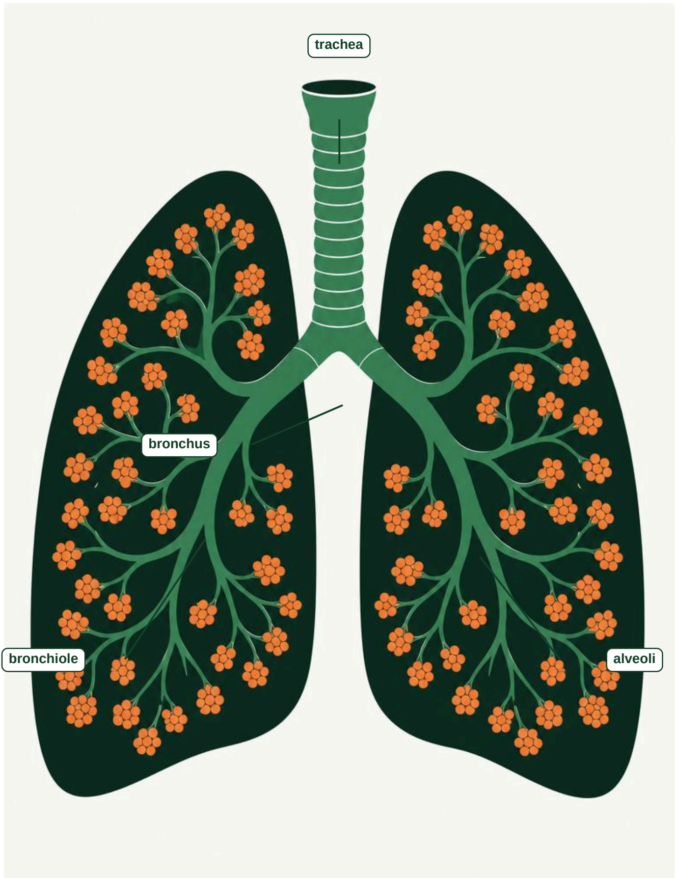
Figure 1.1 The human respiratory system, with the main parts labelled.
