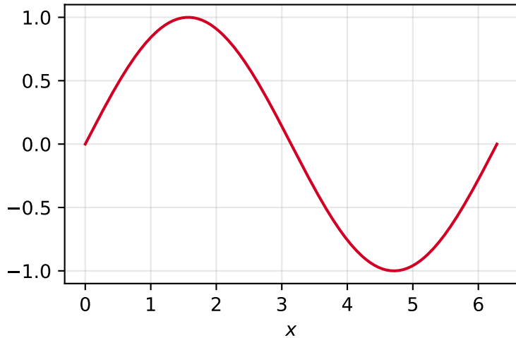
\sin(x)
