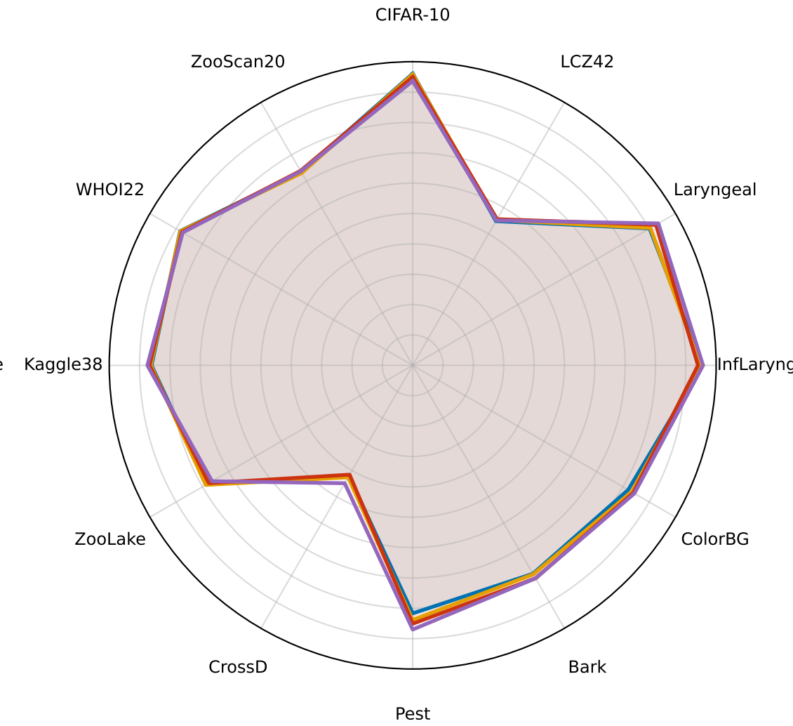
SwinV2
