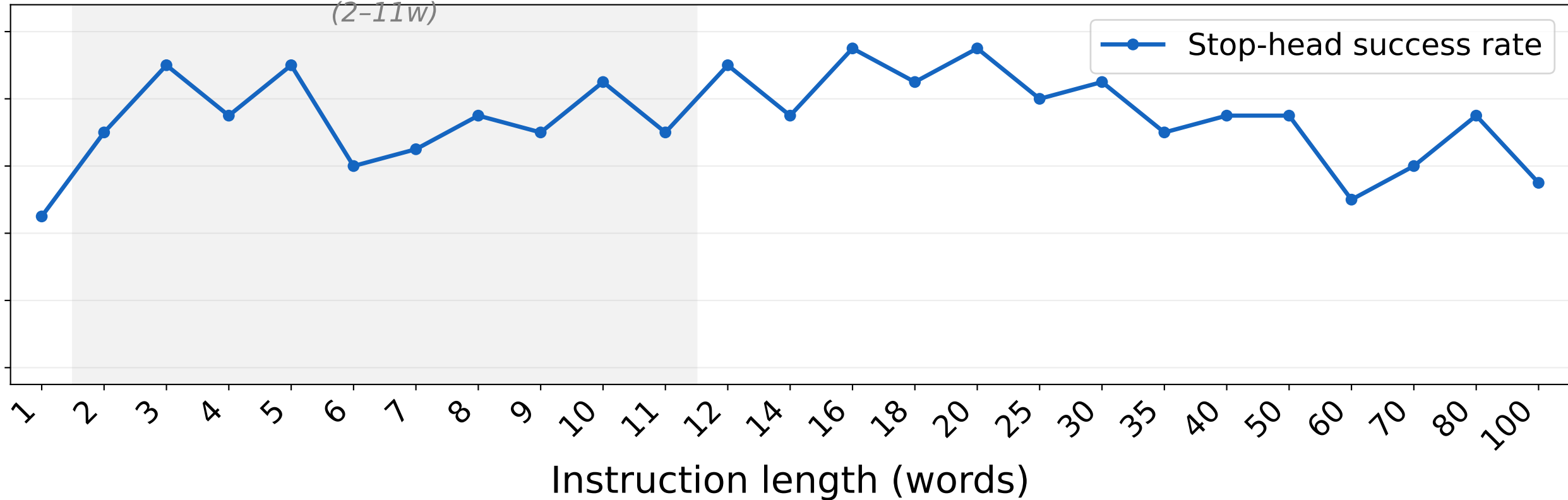
Stop-head success rate vs instruction length
